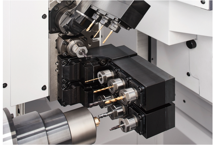
Back machining with the independent back tool post
