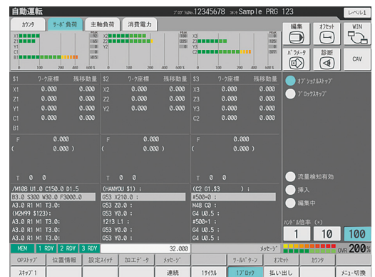
Automatic operation screen Motor load information is displayed graphically, allowing intuitive status checks.
