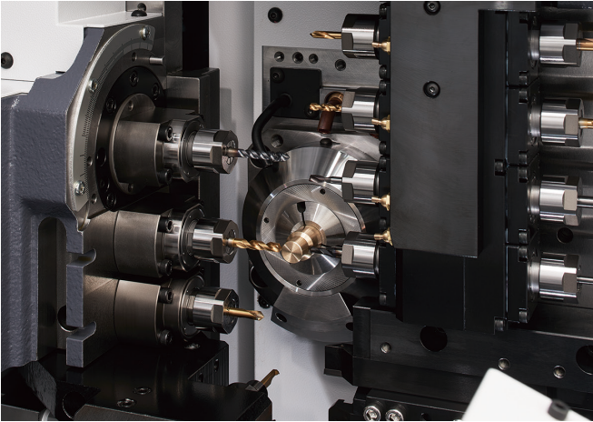
Simultaneous machining with two tools on the front face
